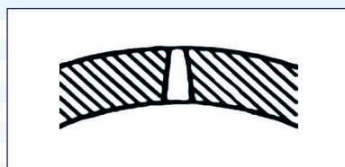
Keystone slot Cut under a 6° angel, this V-shaped slot is non-clogging.
